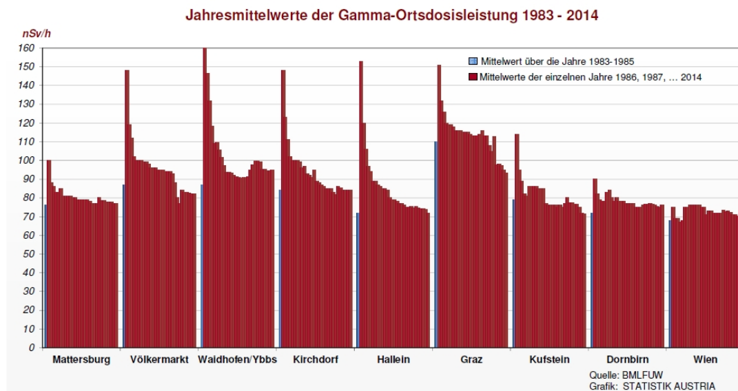
Figure 4: Annual mean values of the gamma-ambient dose rate 1983–2014, source: BMLFUW2015b
